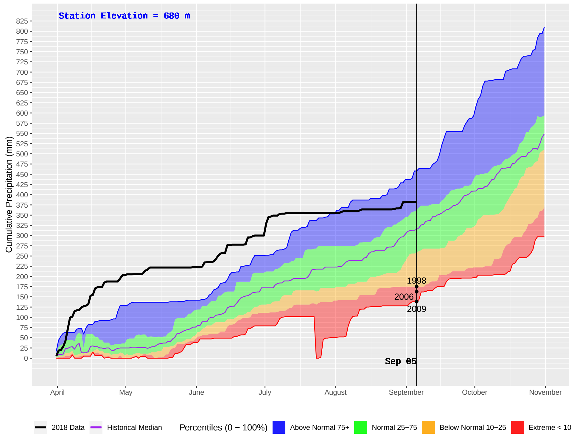
REVELSTOKE (363) : Historical (1995–2016) and Current (2018) Daily Cumulative Precipitation
