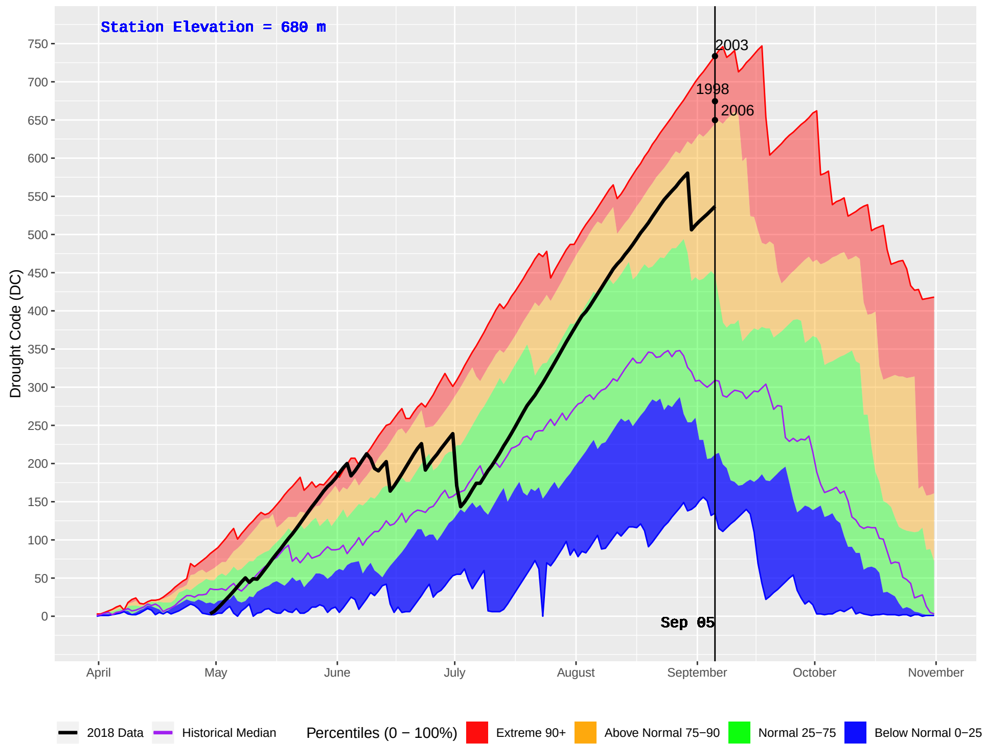
REVELSTOKE (363) : Historical (1995–2016) and Current (2018) Daily Drought Code (DC)
