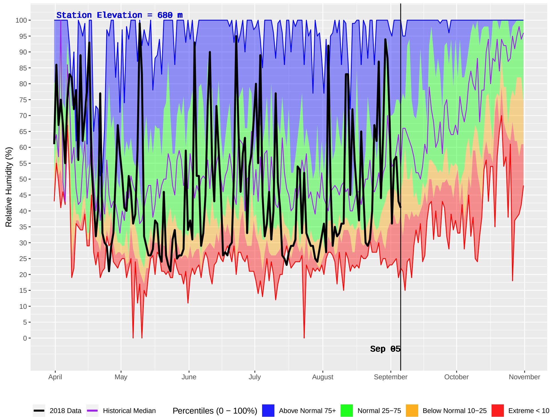
REVELSTOKE (363) : Historical (1995–2016) and Current (2018) Daily Relative Humidity
