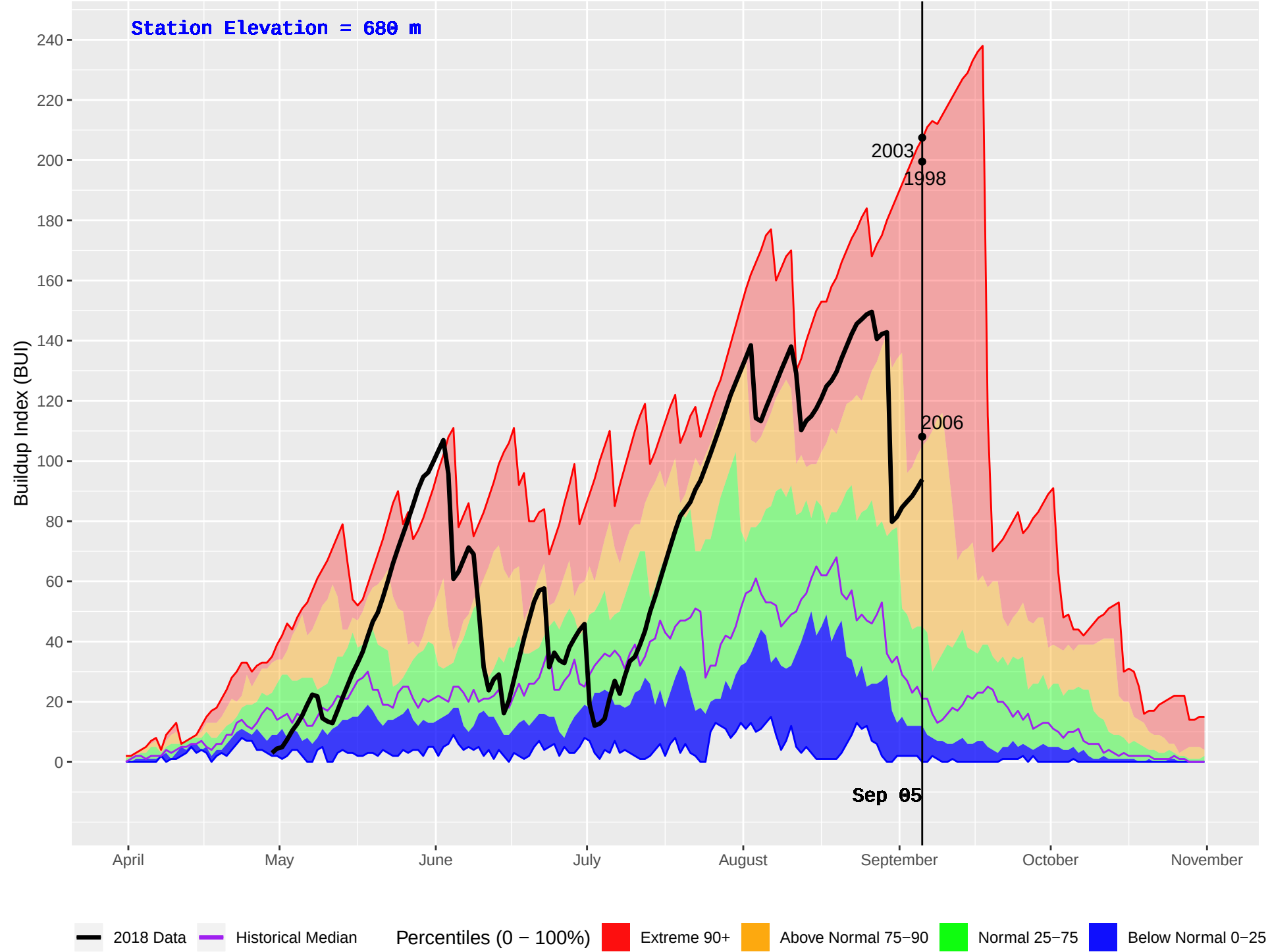
REVELSTOKE (363) : Historical (1995–2016) and Current (2018) Daily Buildup Index (BUI)
