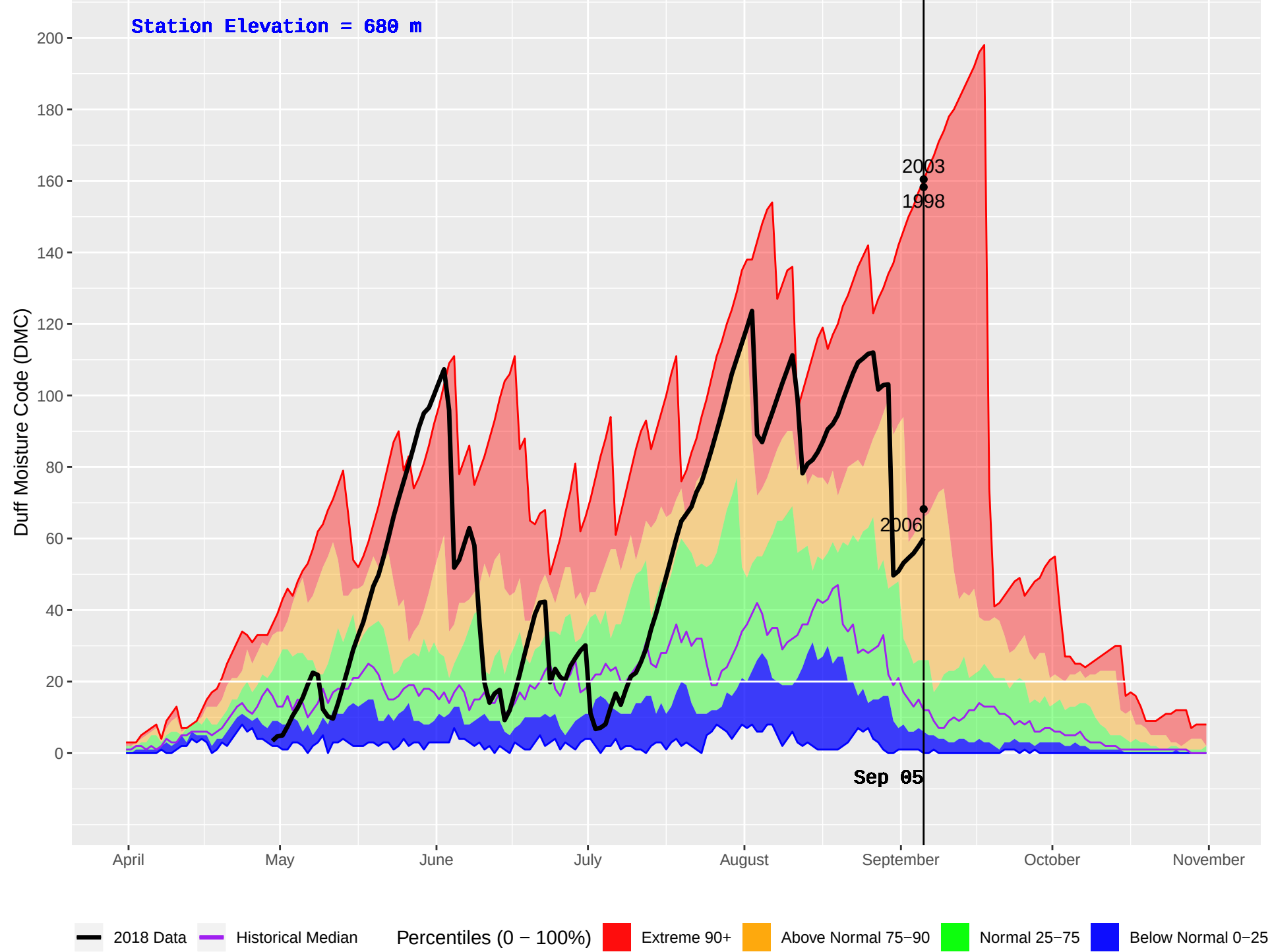
REVELSTOKE (363) : Historical (1995–2016) and Current (2018) Daily Duff Moisture Code (DMC)
