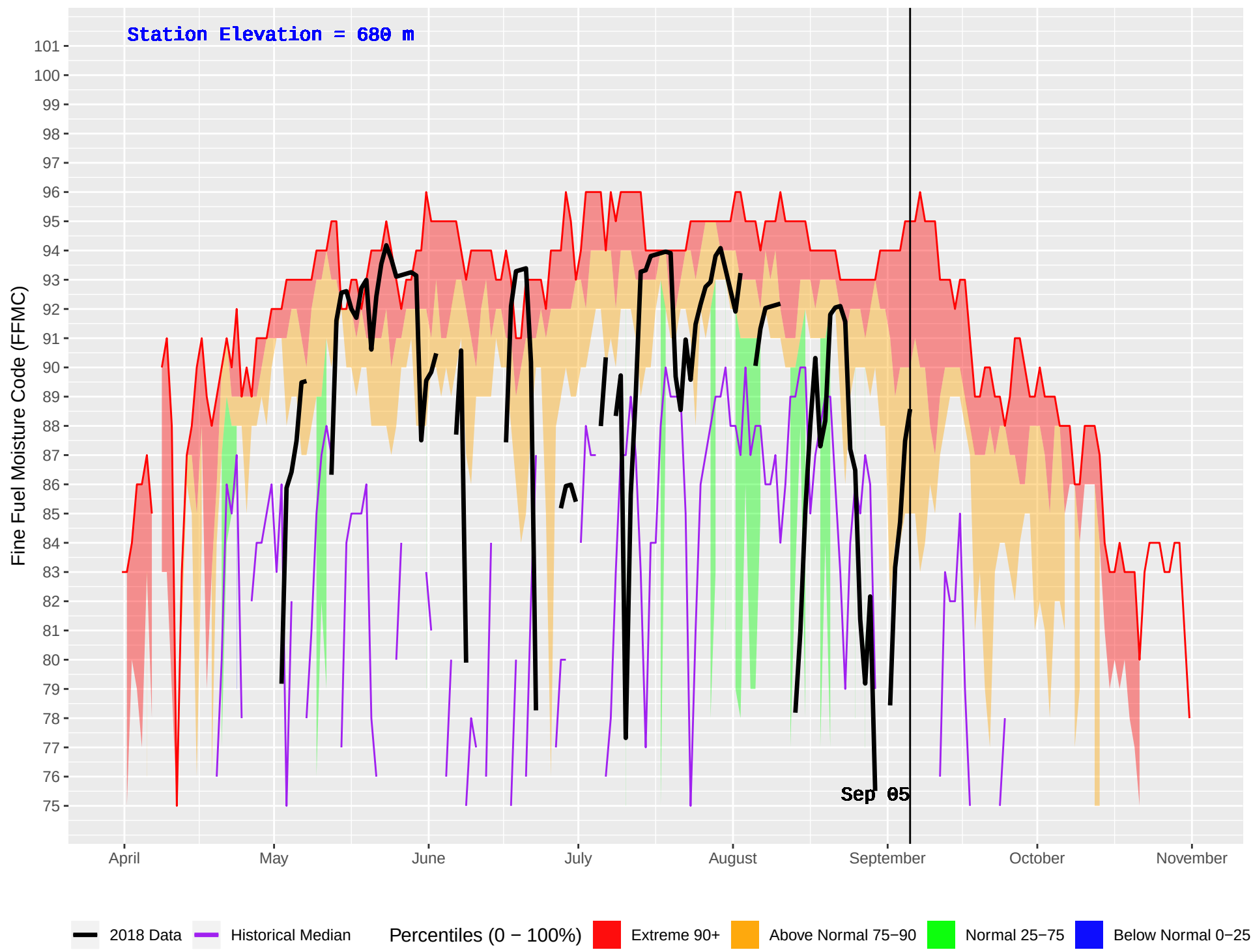
REVELSTOKE (363) : Historical (1995–2016) and Current (2018) Daily Fine Fuel Moisture Code (FFMC)
